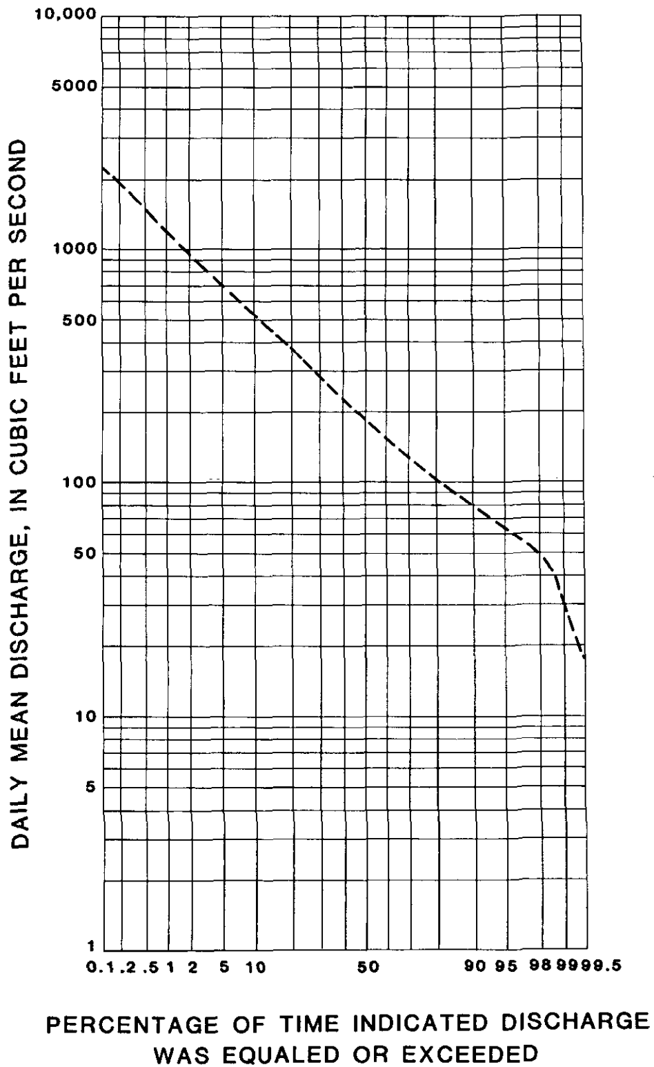
Figure 4.--Flow-duration curve for the Blackstone River at Northbridge, Mass. (site 11), during 1940-77
