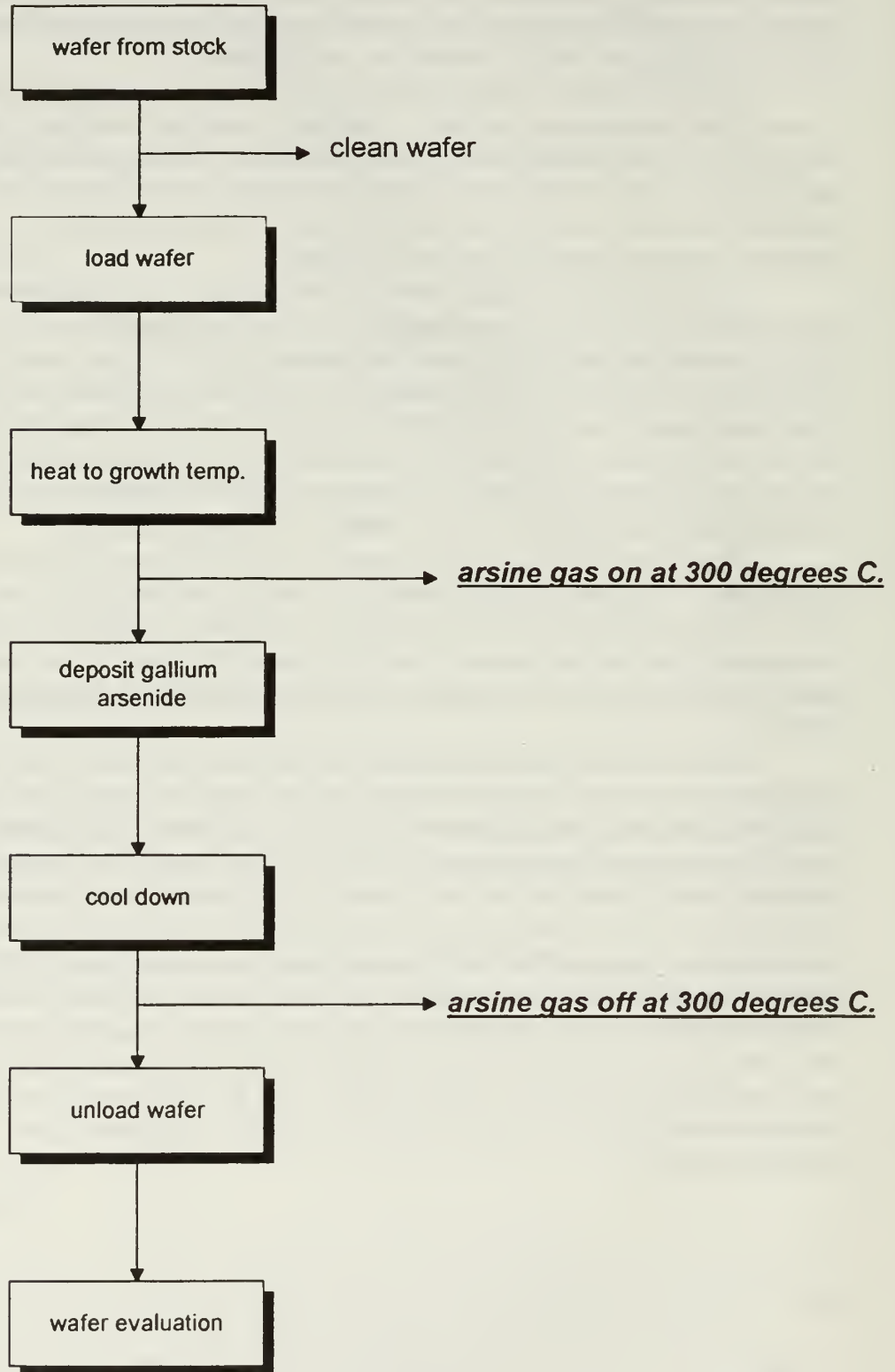
flow diagram 1.
