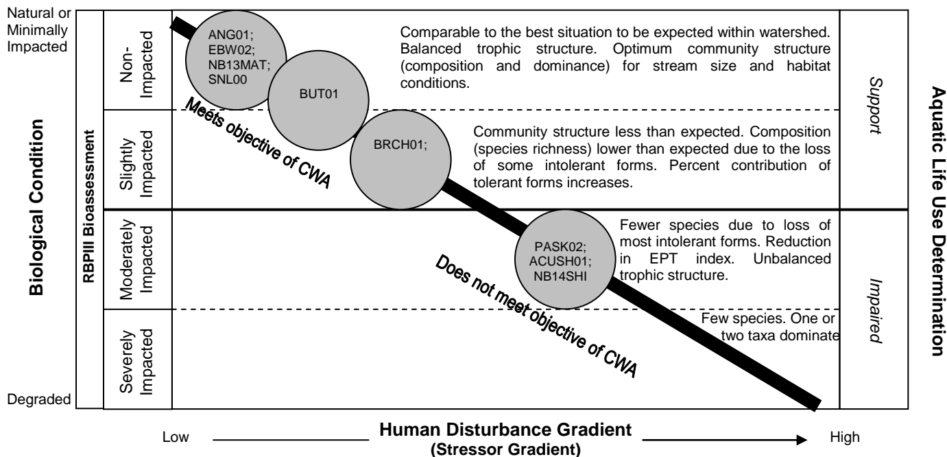
Figure 2. A schematic of results of the RBPIII analysis of the 2005 Buzzards Bay watersheds biomonitoring stations as they relate to Tiered Aquatic Life Use.
